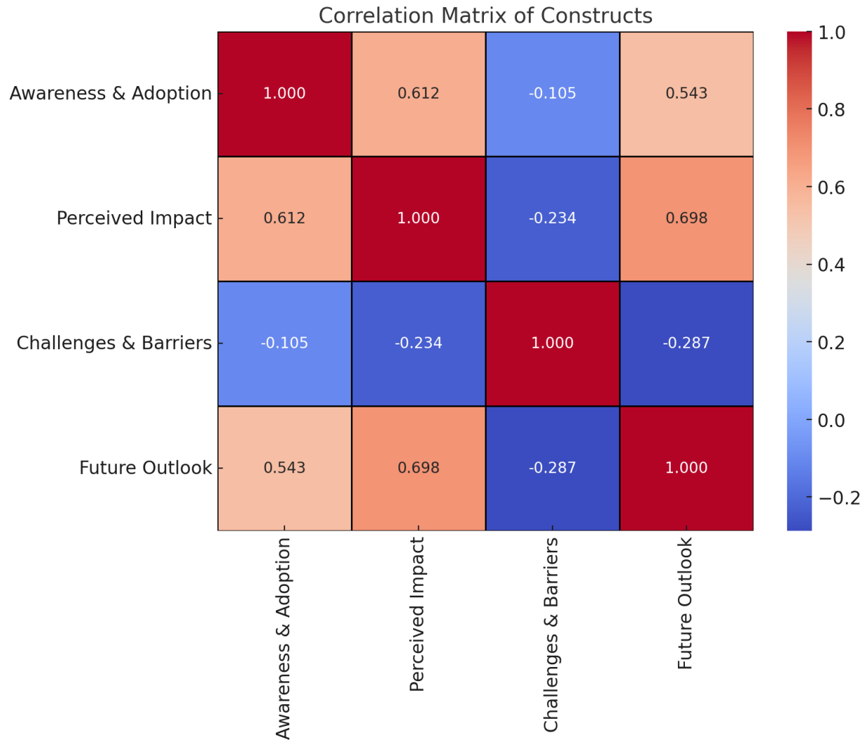
Figure 4: Correlation Analysis
